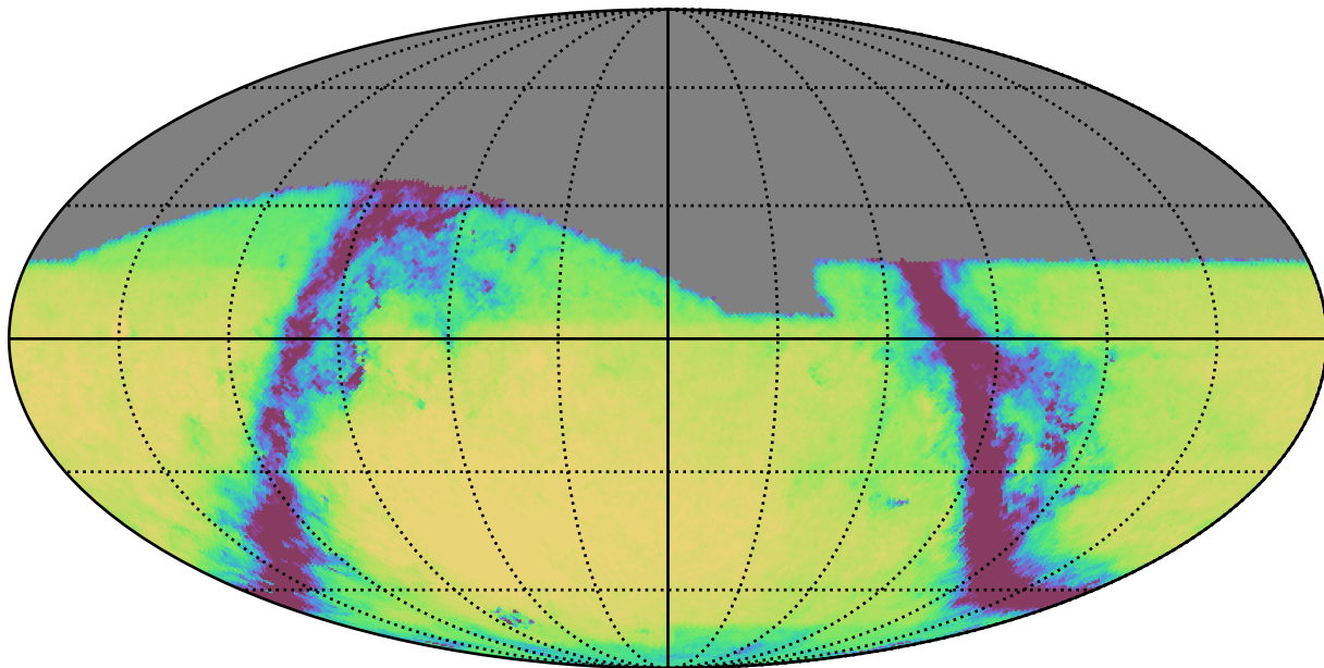
baseline_v2.0_10yrs All sky g band: Exgal_CoaddM5
