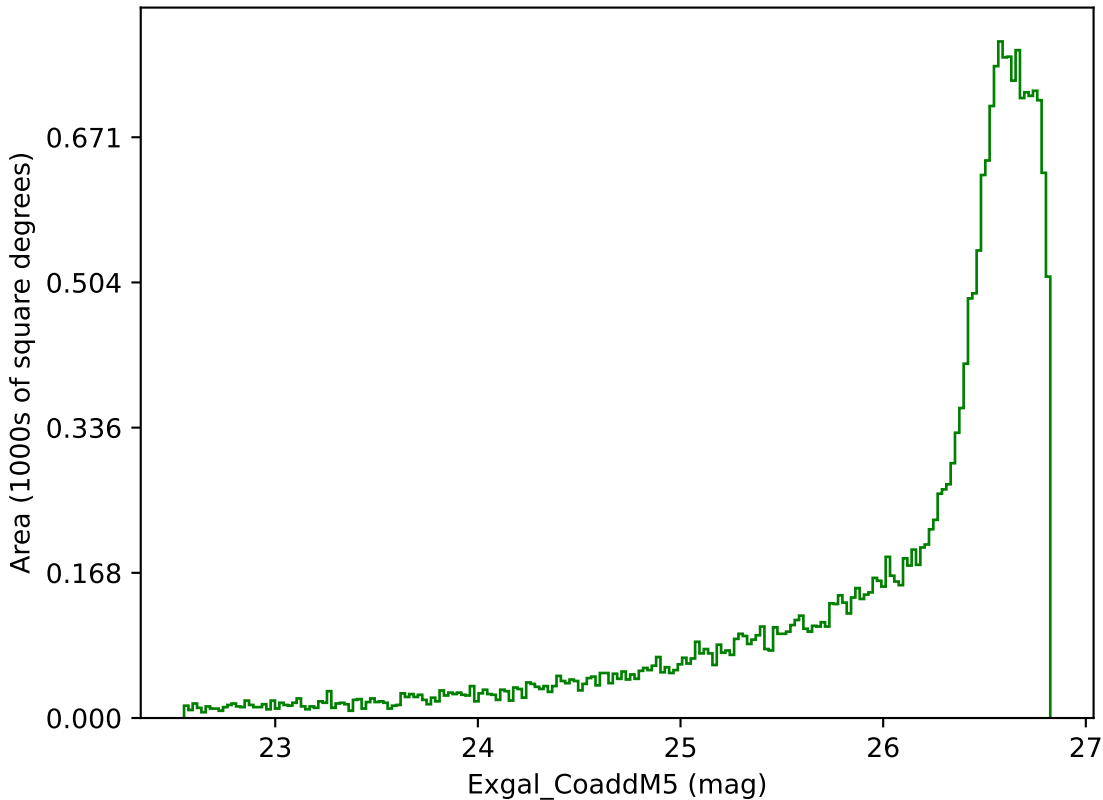
baseline_v2.0_10yrs All sky g band: Exgal_CoaddM5
