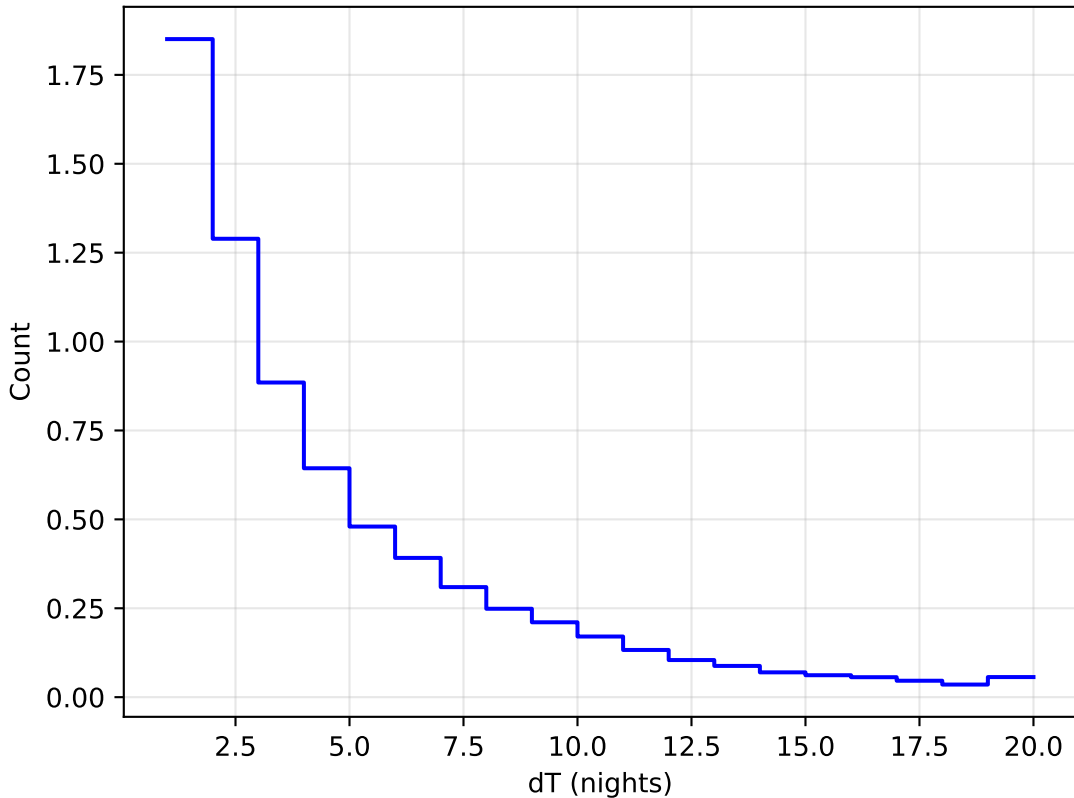
baseline_v2.0_10yrs WFD all bands: DeltaNight Histogram 1e6
