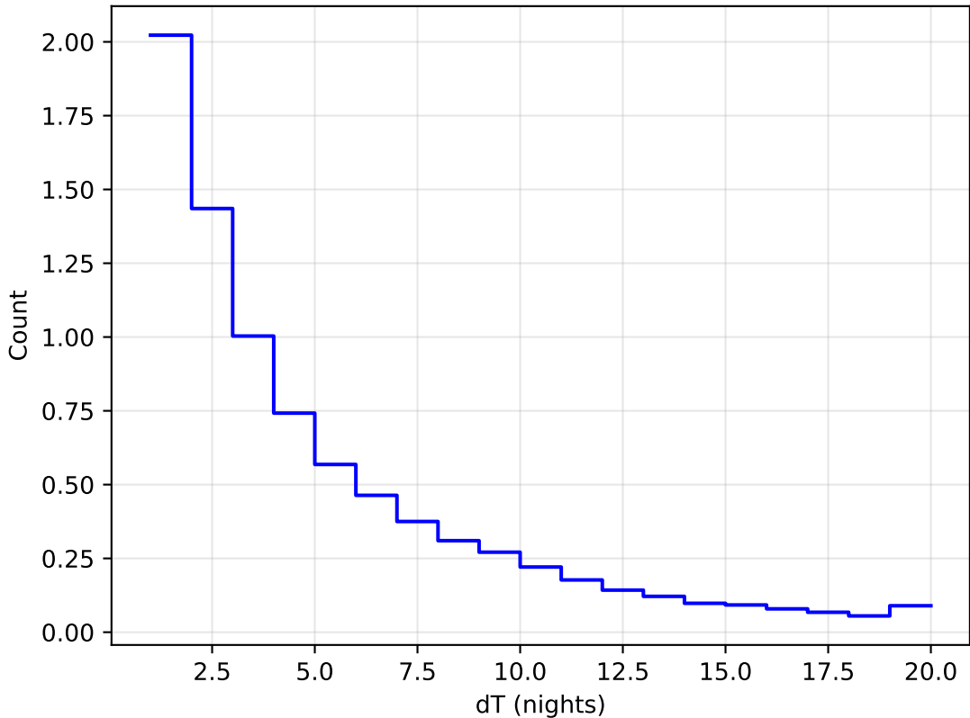
baseline_v2.0_10yrs All sky all bands: DeltaNight Histogram 1e6
