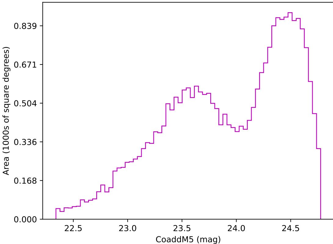
baseline_v2.0_10yrs Yr 3-4 z band: CoaddM5
