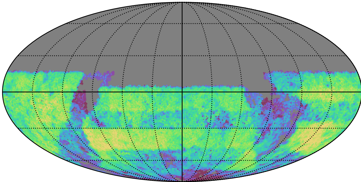
baseline_v2.0_10yrs Yr 3-4 u band: CoaddM5
