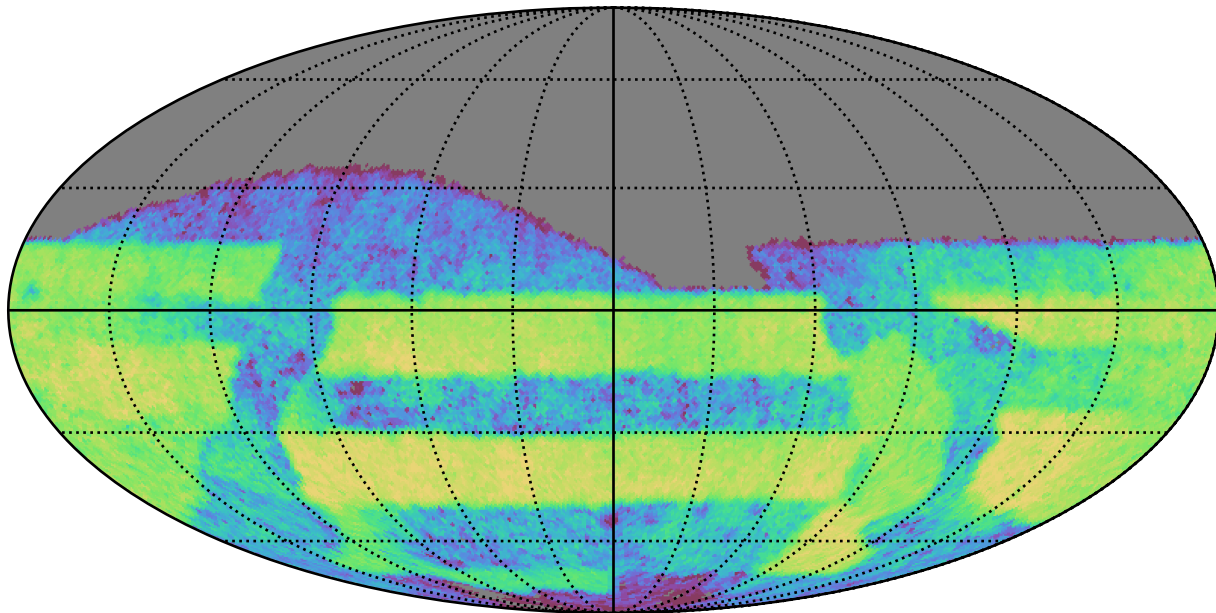
baseline_v2.0_10yrs Yr 3-4 r band: CoaddM5
