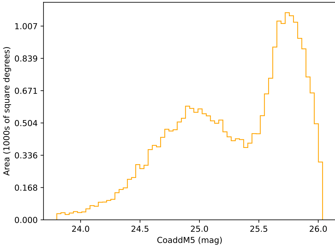
baseline_v2.0_10yrs Yr 3-4 r band: CoaddM5
