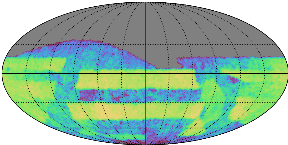
baseline_v2.0_10yrs Yr 3-4 i band: CoaddM5
