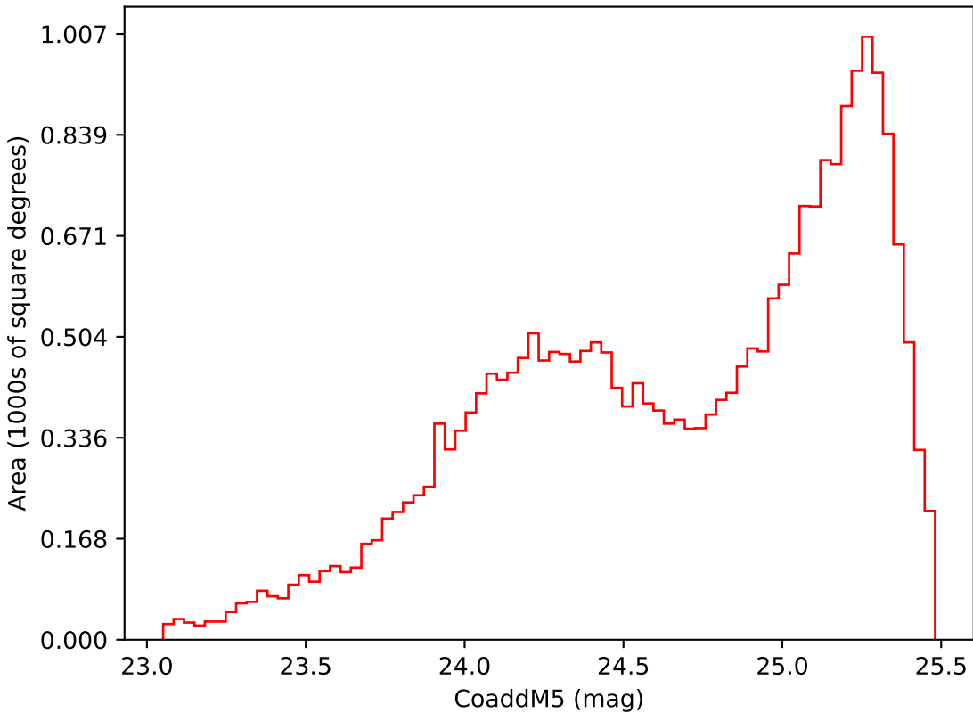
baseline_v2.0_10yrs Yr 3-4 i band: CoaddM5
