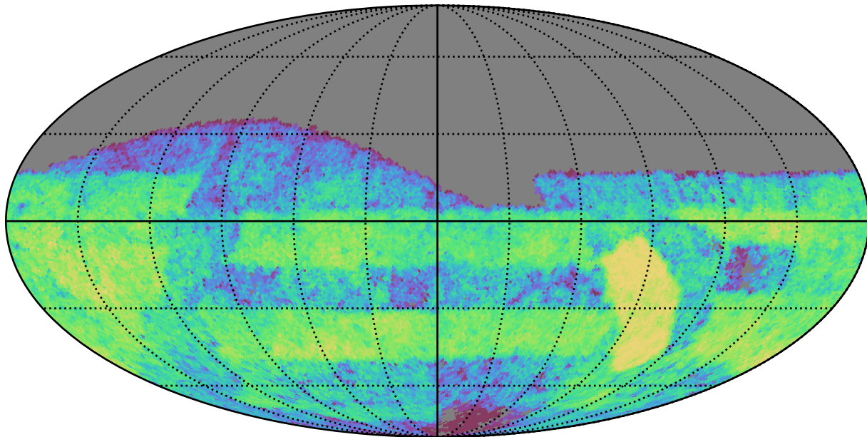
baseline_v2.0_10yrs Yr 3-4 g band: CoaddM5
