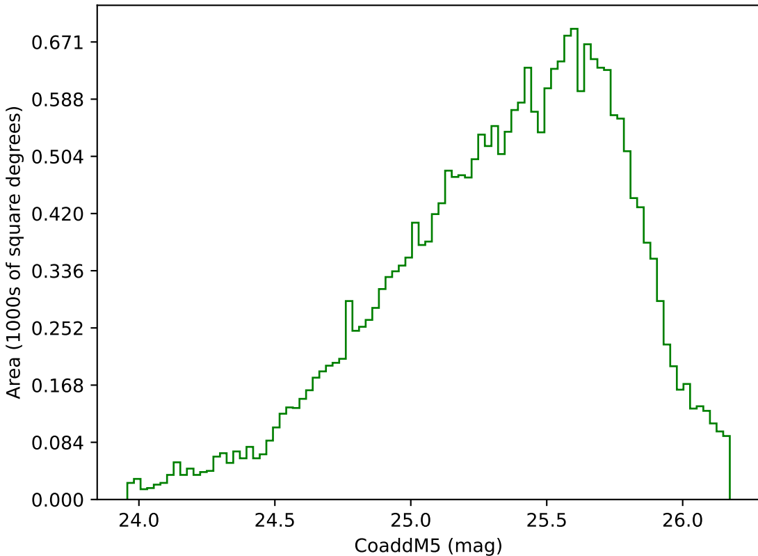
baseline_v2.0_10yrs Yr 3-4 g band: CoaddM5
