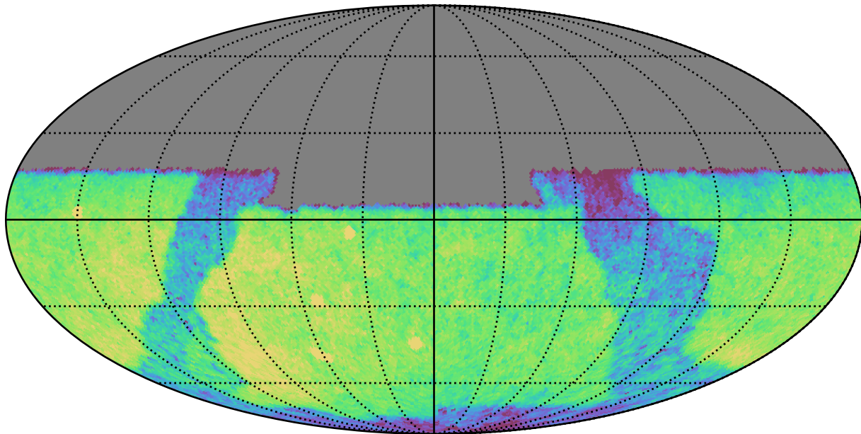
baseline_v2.0_10yrs Yr 1 y band: CoaddM5
