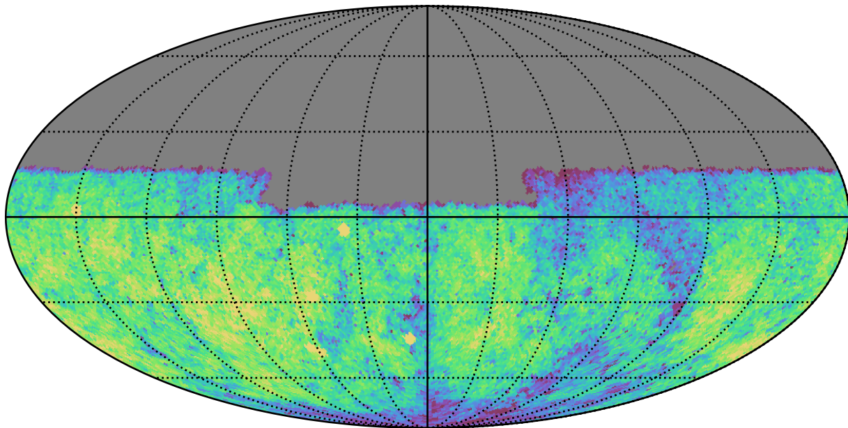
baseline_v2.0_10yrs Yr 1 u band: CoaddM5
