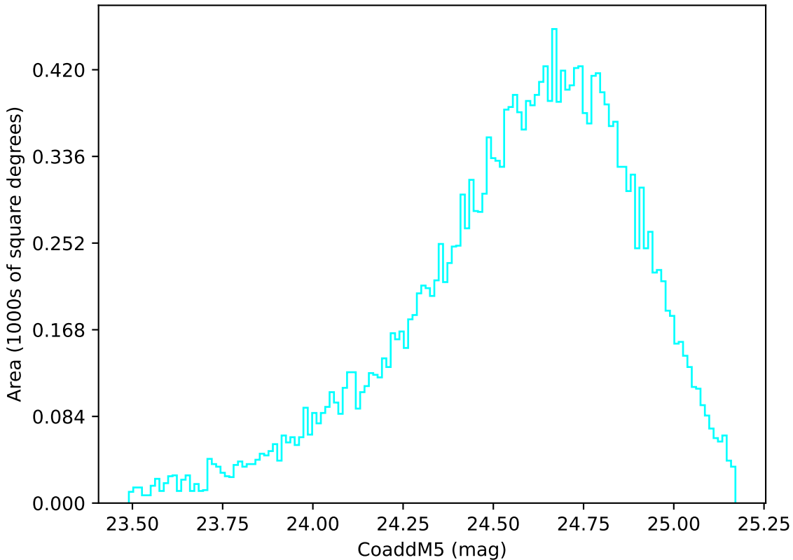
baseline_v2.0_10yrs Yr 1 u band: CoaddM5
