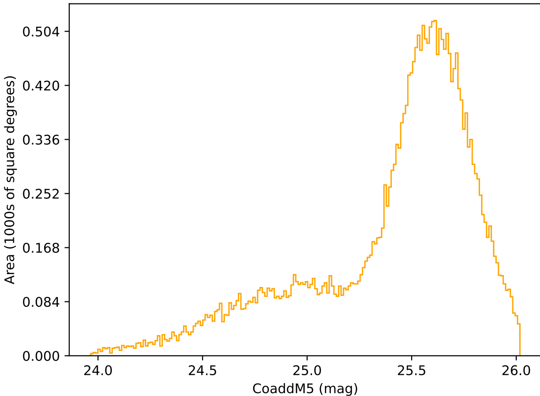
baseline_v2.0_10yrs Yr 1 r band: CoaddM5
