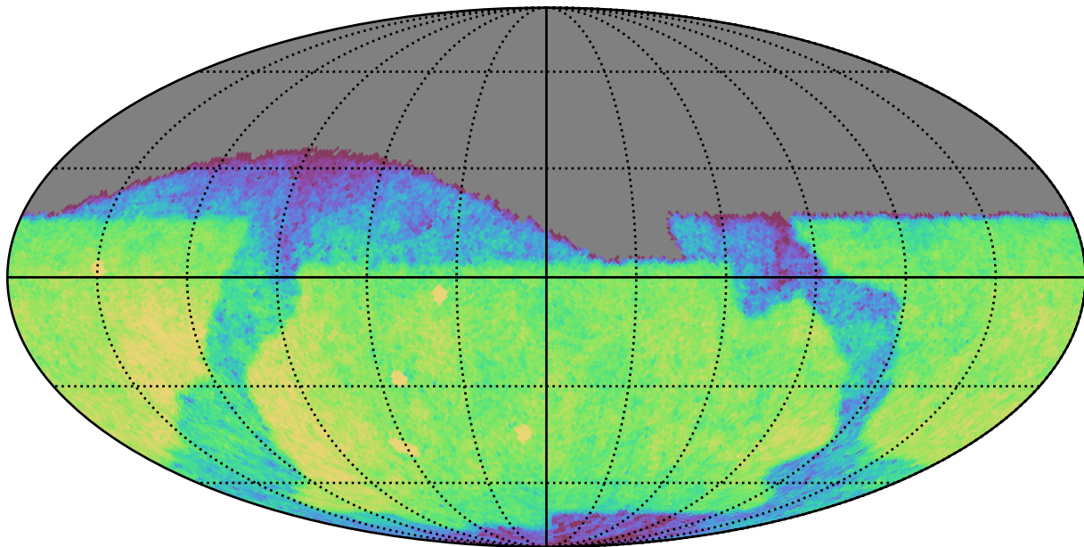
baseline_v2.0_10yrs Yr 1 i band: CoaddM5
