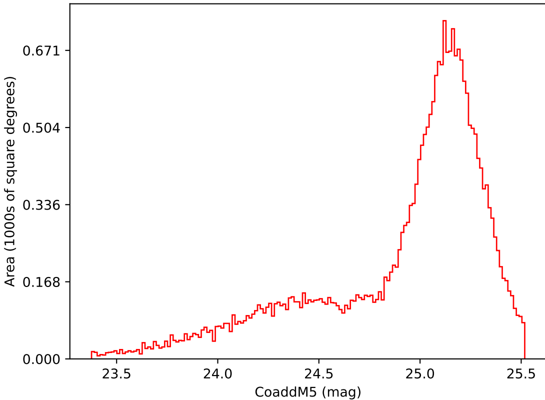
baseline_v2.0_10yrs Yr 1 i band: CoaddM5
