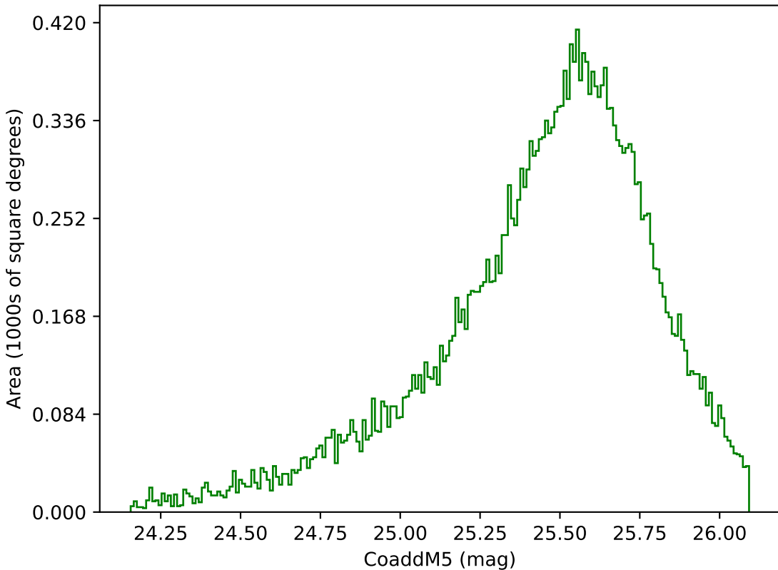
baseline_v2.0_10yrs Yr 1 g band: CoaddM5
