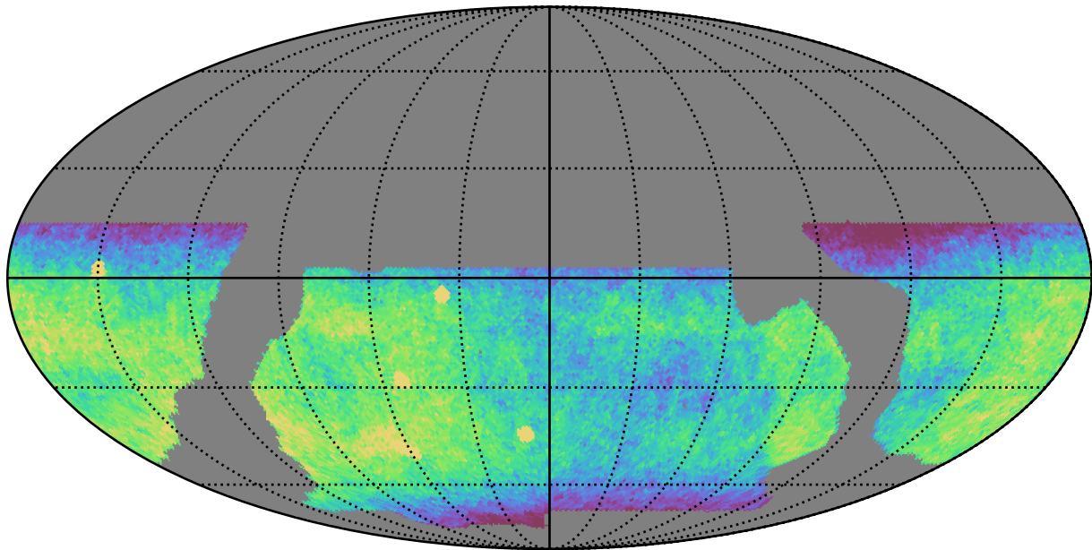
baseline_v2.0_10yrs WFD z band: CoaddM5
