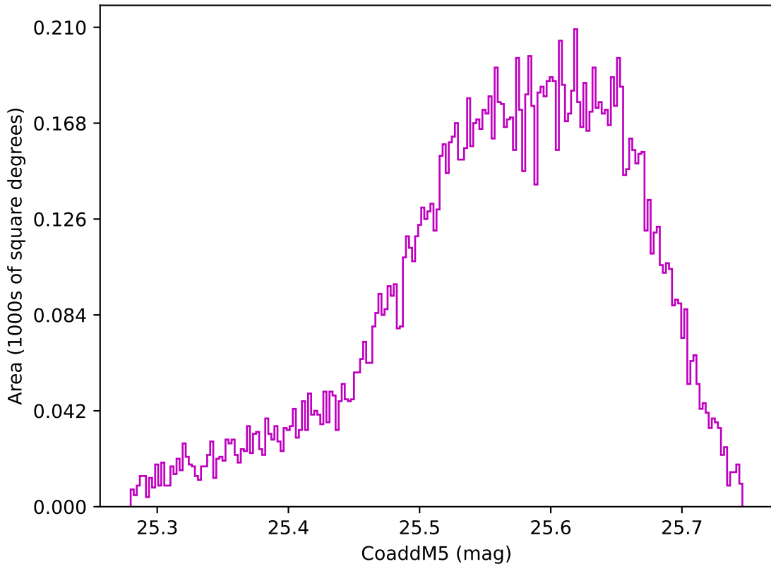
baseline_v2.0_10yrs WFD z band: CoaddM5
