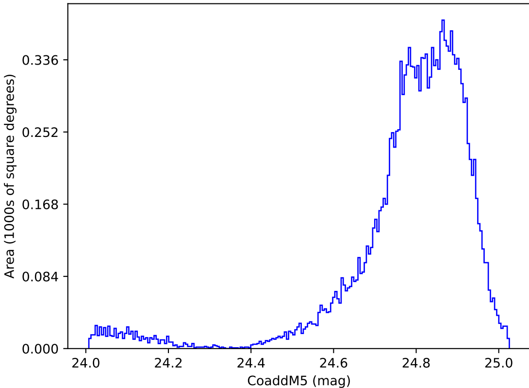
baseline_v2.0_10yrs WFD y band: CoaddM5
