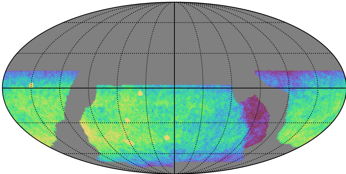
baseline_v2.0_10yrs WFD u band: CoaddM5
