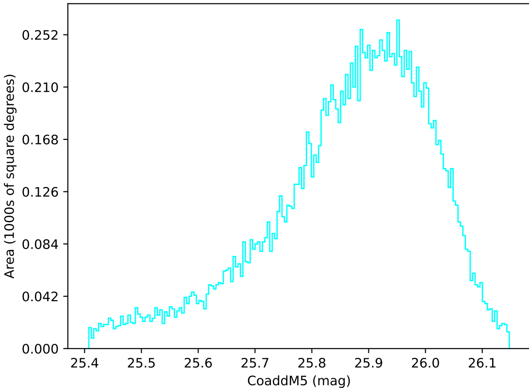
baseline_v2.0_10yrs WFD u band: CoaddM5
