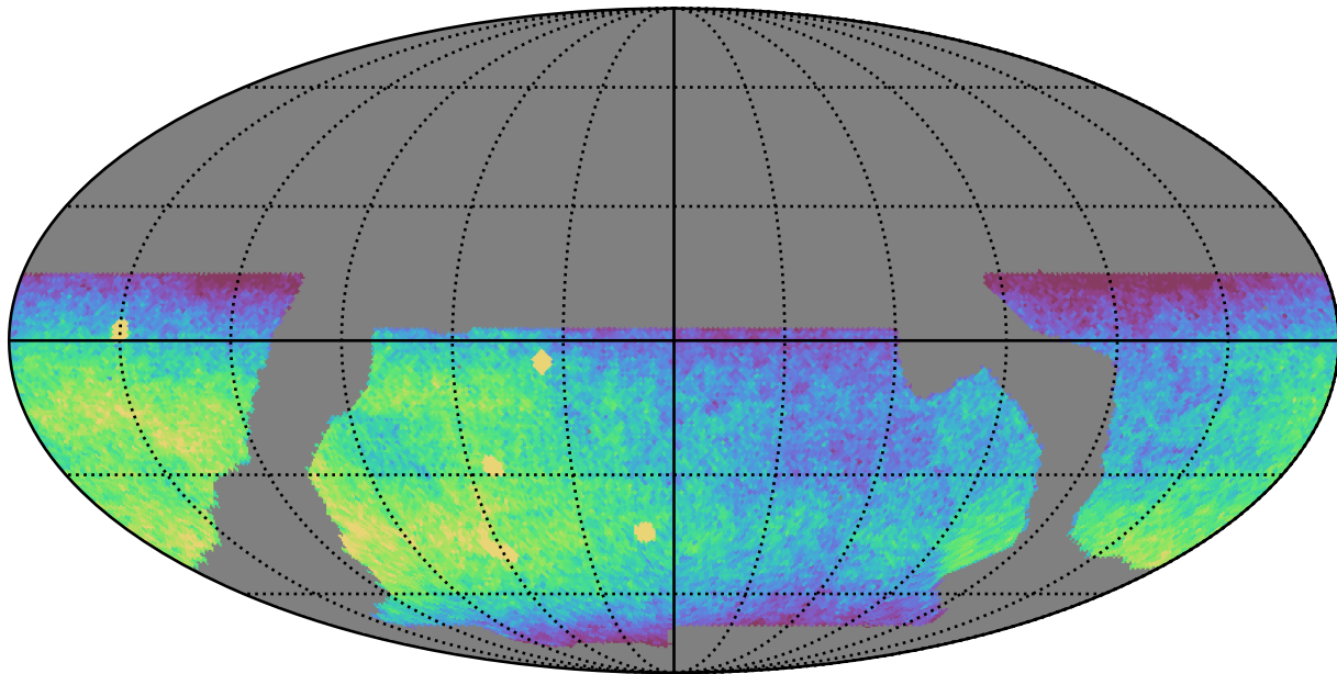
baseline_v2.0_10yrs WFD r band: CoaddM5
