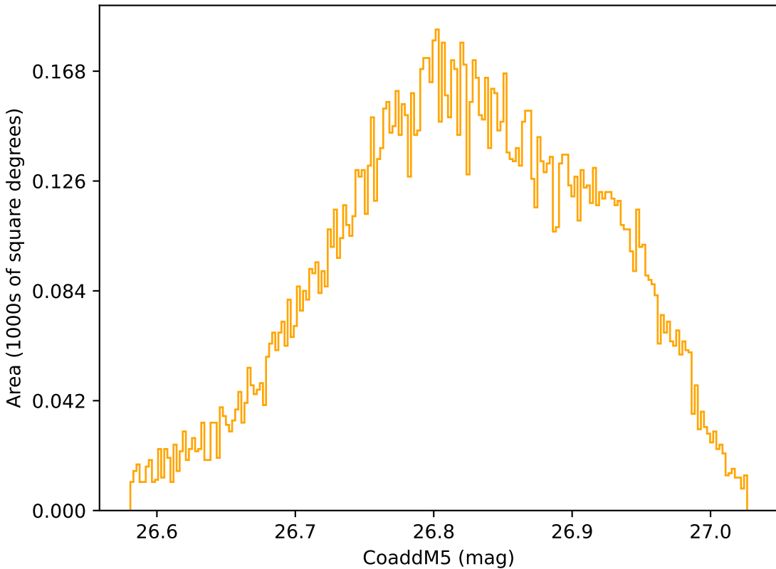
baseline_v2.0_10yrs WFD r band: CoaddM5
