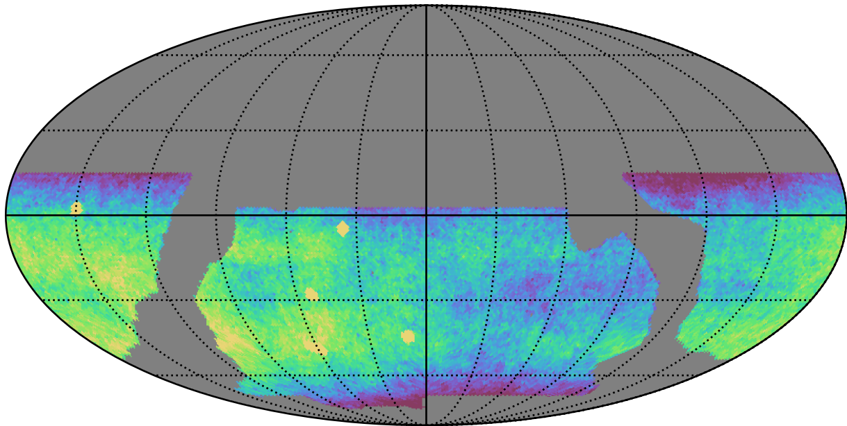
baseline_v2.0_10yrs WFD i band: CoaddM5
