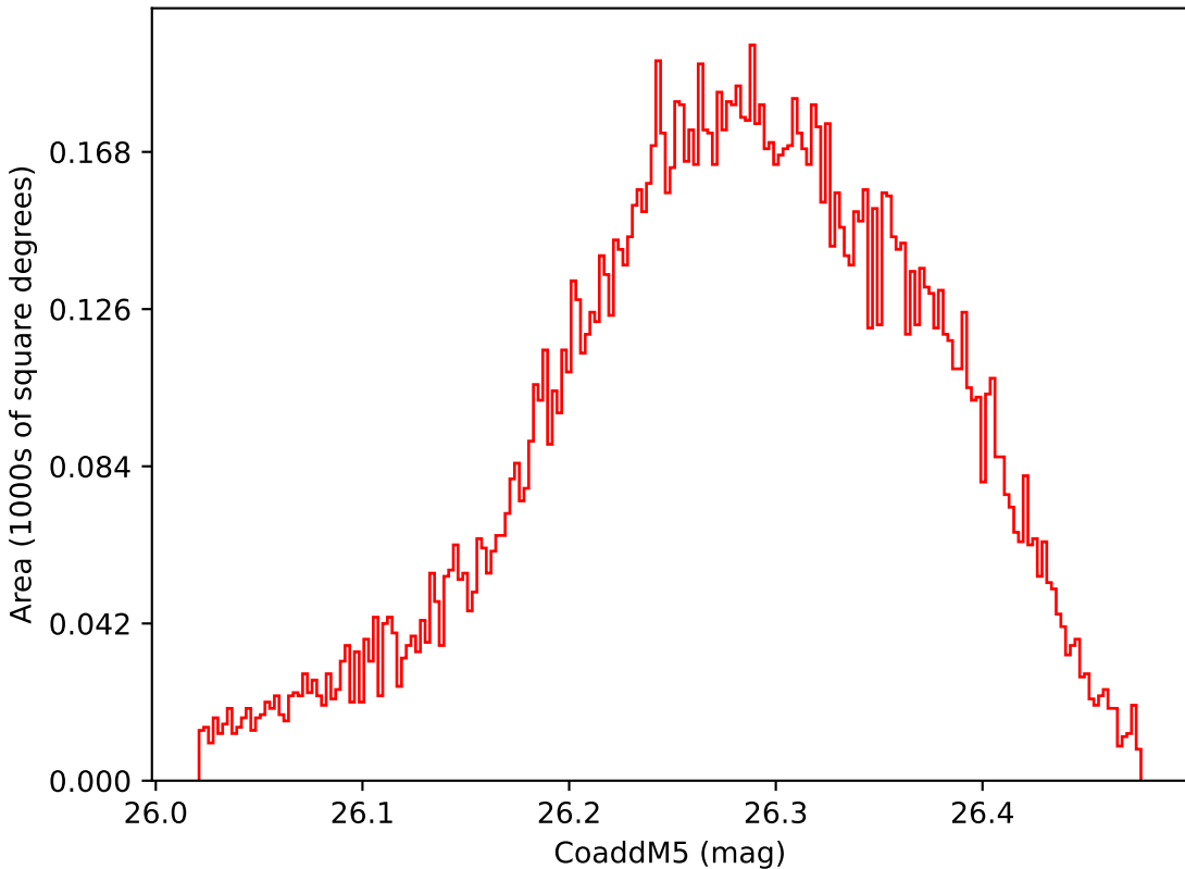
baseline_v2.0_10yrs WFD i band: CoaddM5
