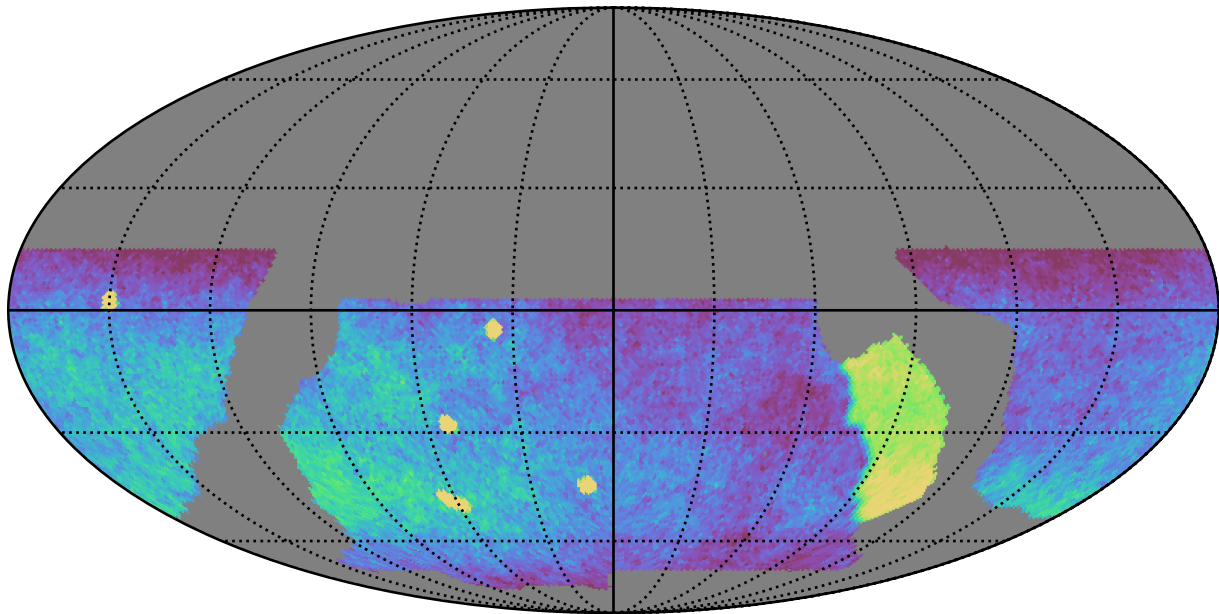
baseline_v2.0_10yrs WFD g band: CoaddM5
