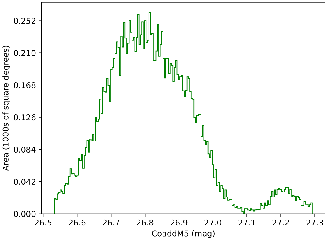
baseline_v2.0_10yrs WFD g band: CoaddM5
