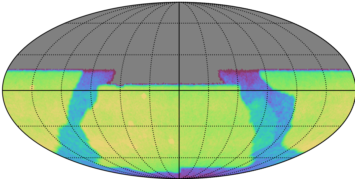
baseline_v2.0_10yrs All sky y band: CoaddM5
