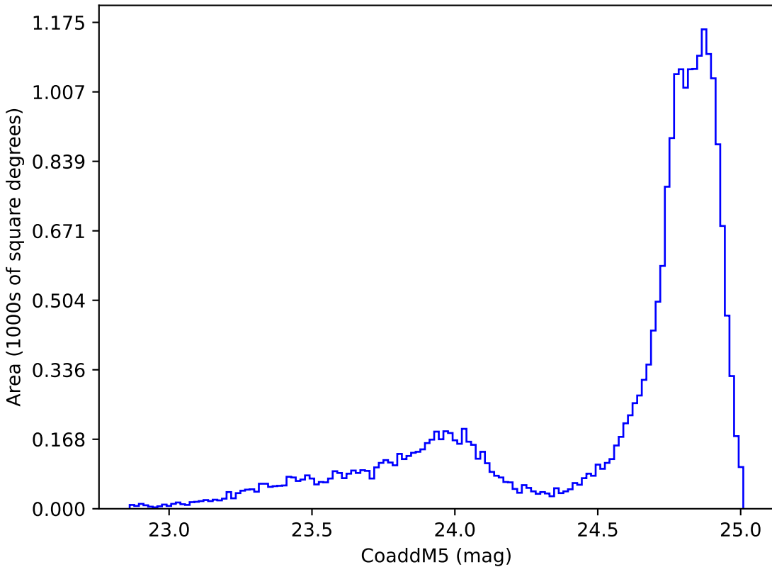
baseline_v2.0_10yrs All sky y band: CoaddM5
