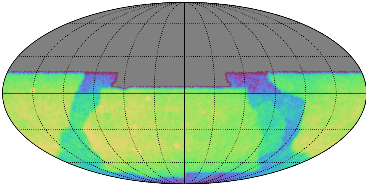
baseline_v2.0_10yrs All sky u band: CoaddM5
