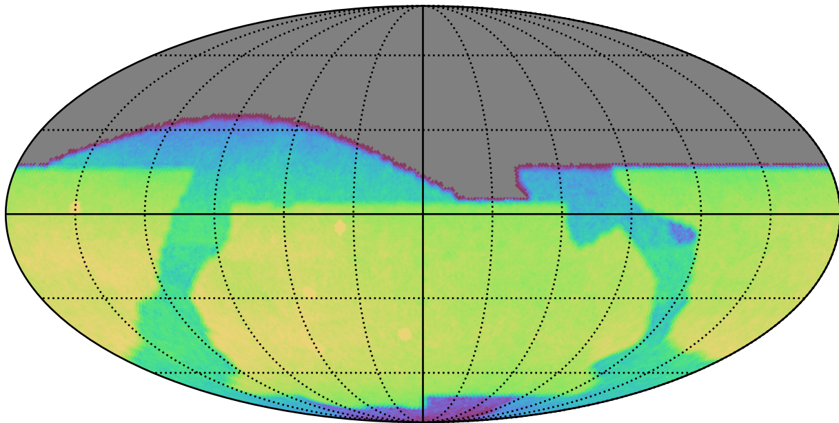
baseline_v2.0_10yrs All sky r band: CoaddM5
