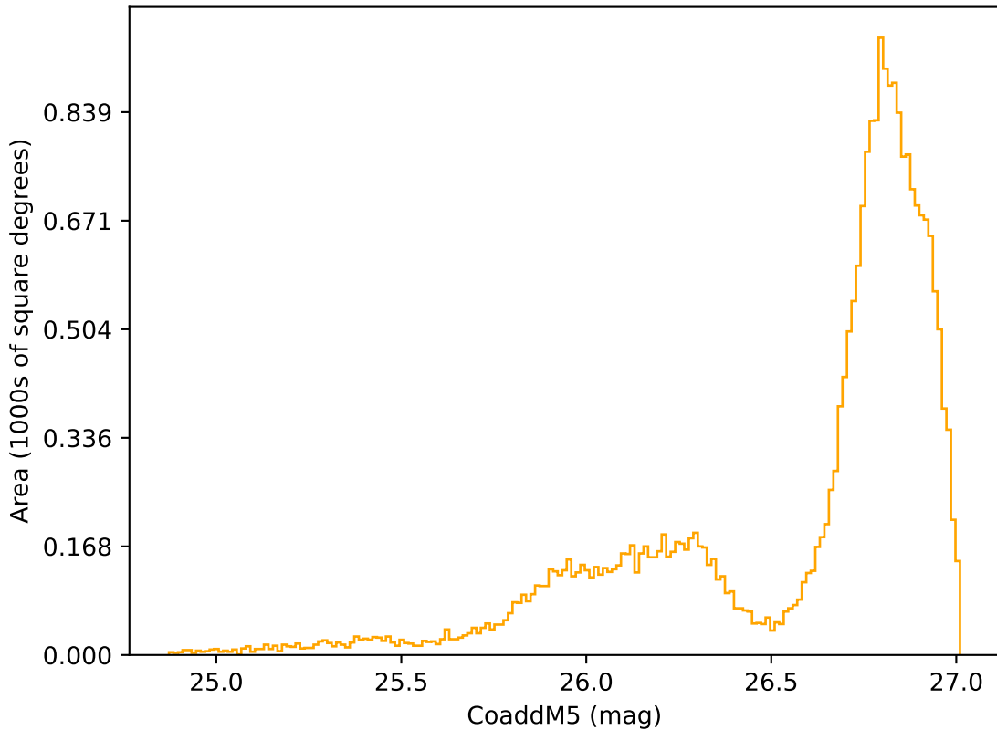
baseline_v2.0_10yrs All sky r band: CoaddM5
