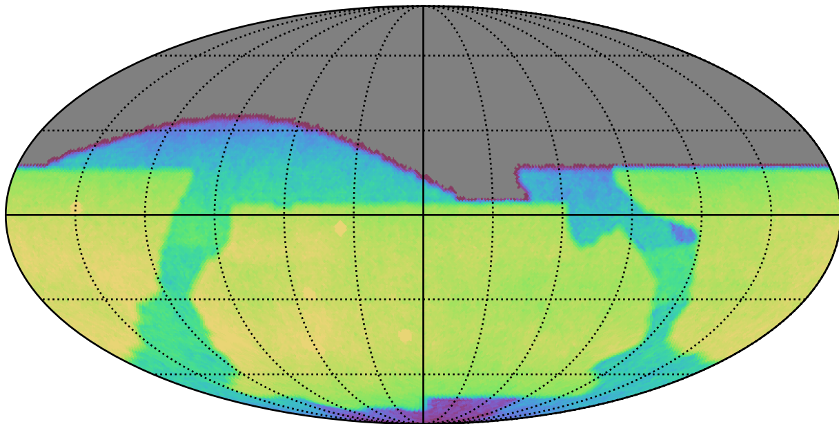
baseline_v2.0_10yrs All sky i band: CoaddM5
