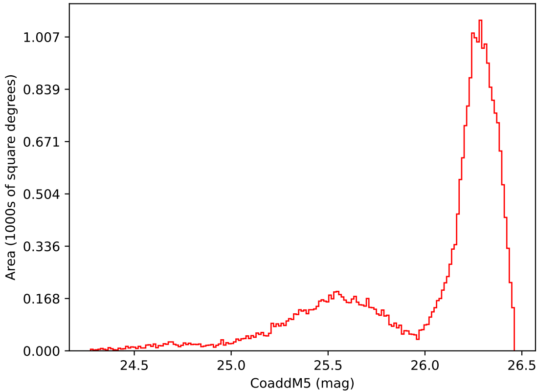
baseline_v2.0_10yrs All sky i band: CoaddM5
