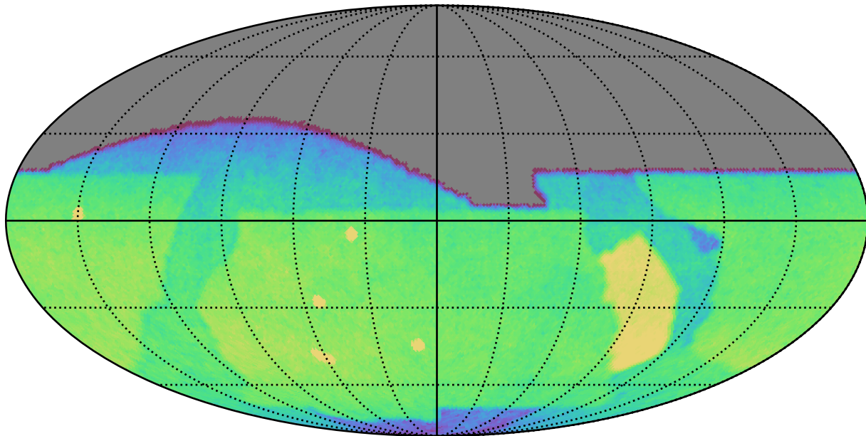
baseline_v2.0_10yrs All sky g band: CoaddM5
