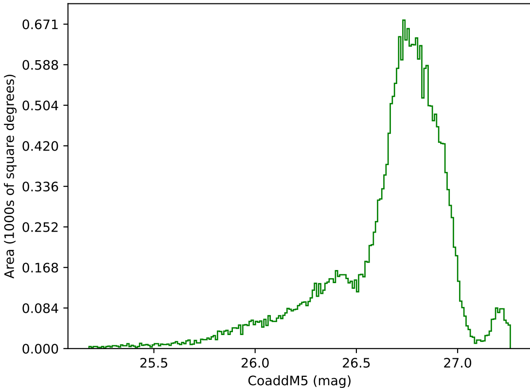
baseline_v2.0_10yrs All sky g band: CoaddM5
