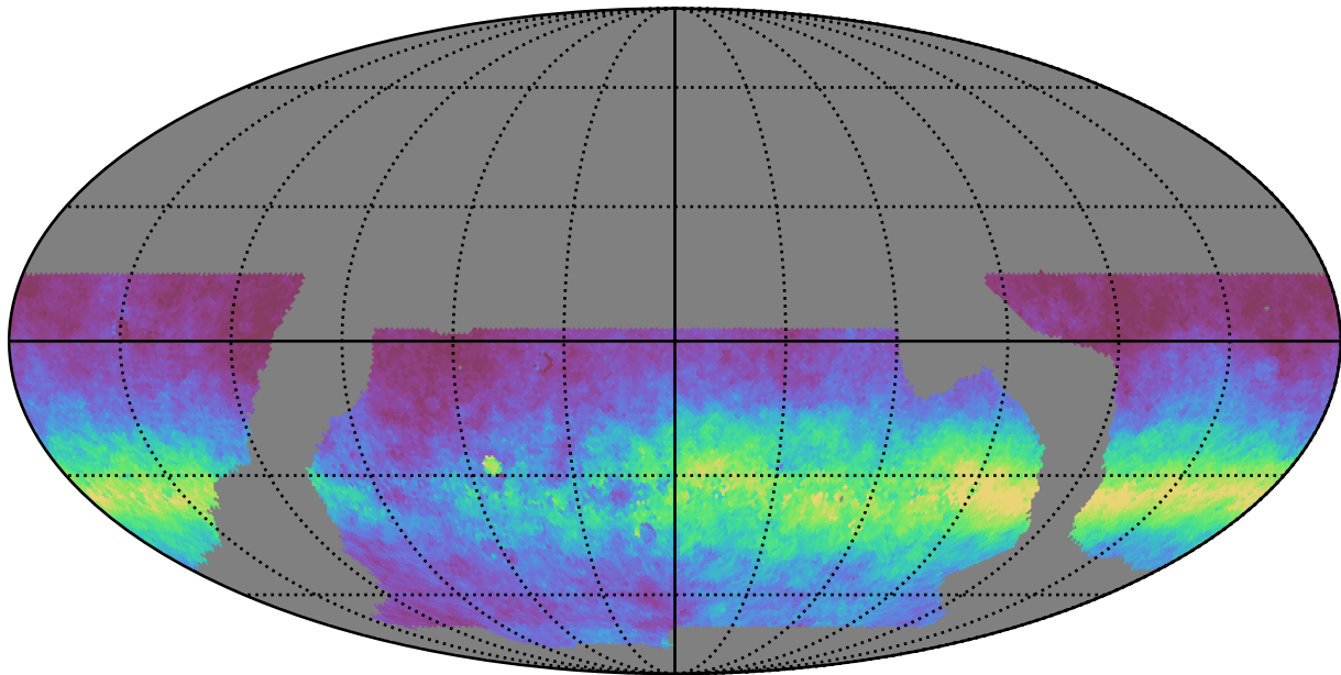
baseline_v2.0_10yrs WFD z band: AngleRms rotSkyPos
