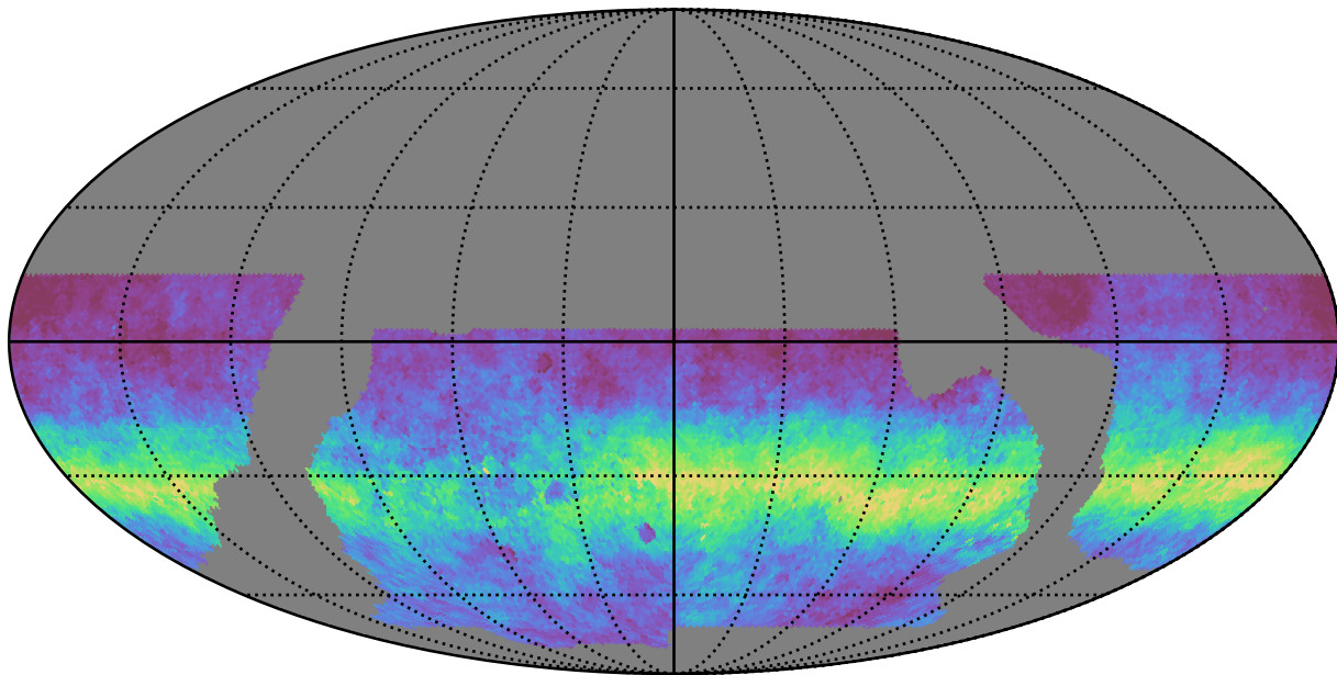
baseline_v2.0_10yrs WFD u band: AngleRms rotSkyPos
