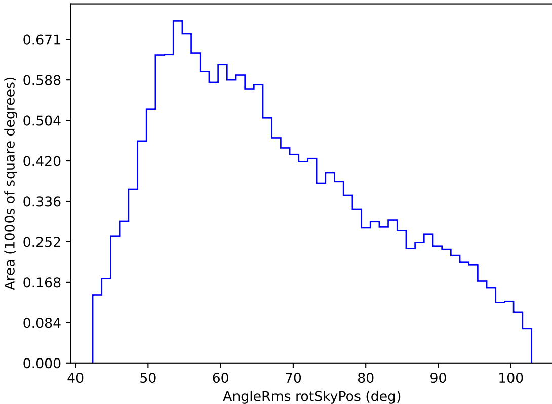
baseline_v2.0_10yrs WFD u band: AngleRms rotSkyPos
