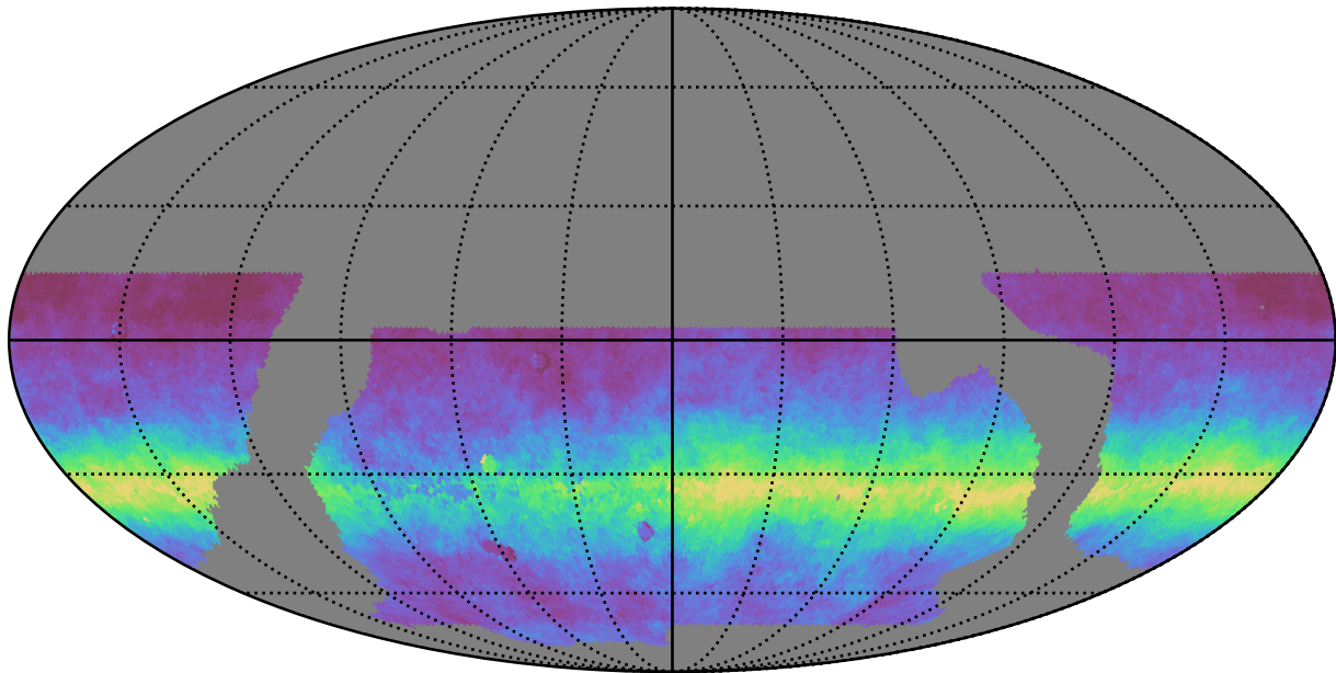
baseline_v2.0_10yrs WFD r band: AngleRms rotSkyPos
