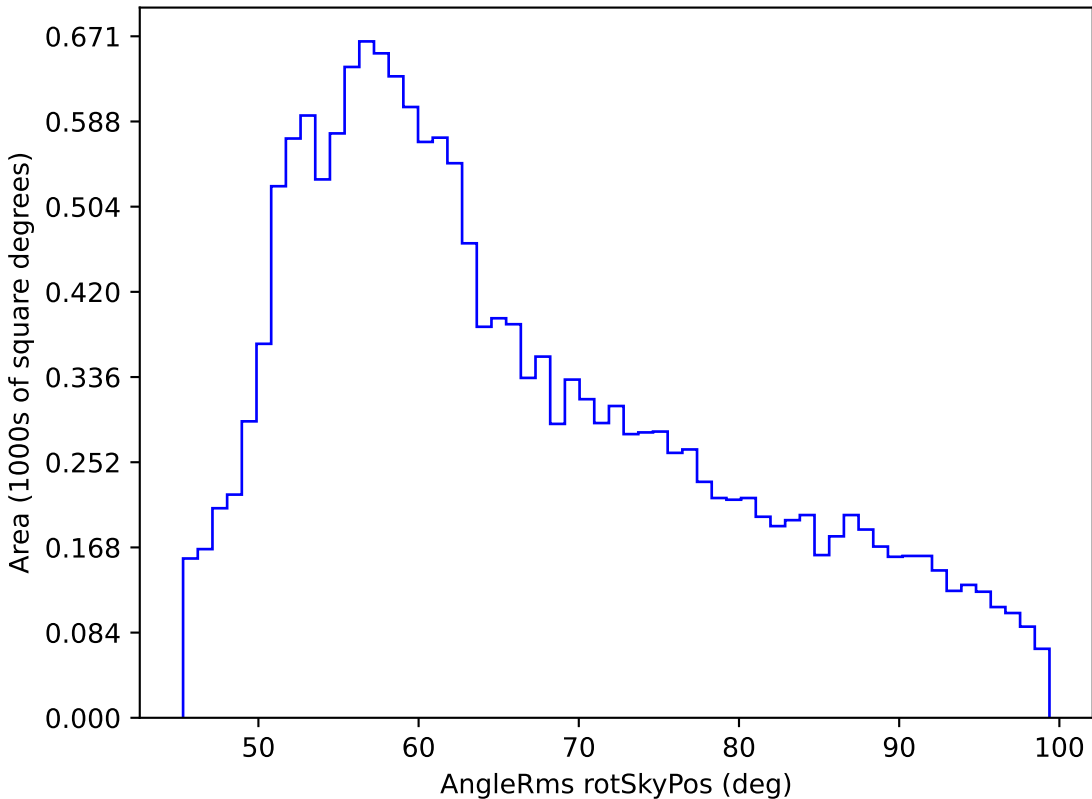
baseline_v2.0_10yrs WFD r band: AngleRms rotSkyPos
