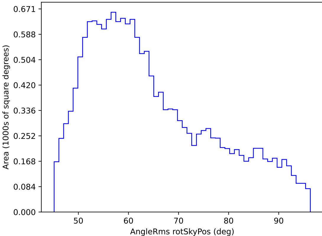
baseline_v2.0_10yrs WFD i band: AngleRms rotSkyPos
