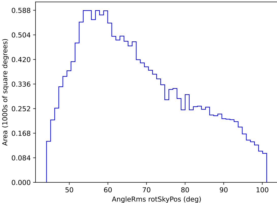
baseline_v2.0_10yrs WFD g band: AngleRms rotSkyPos
