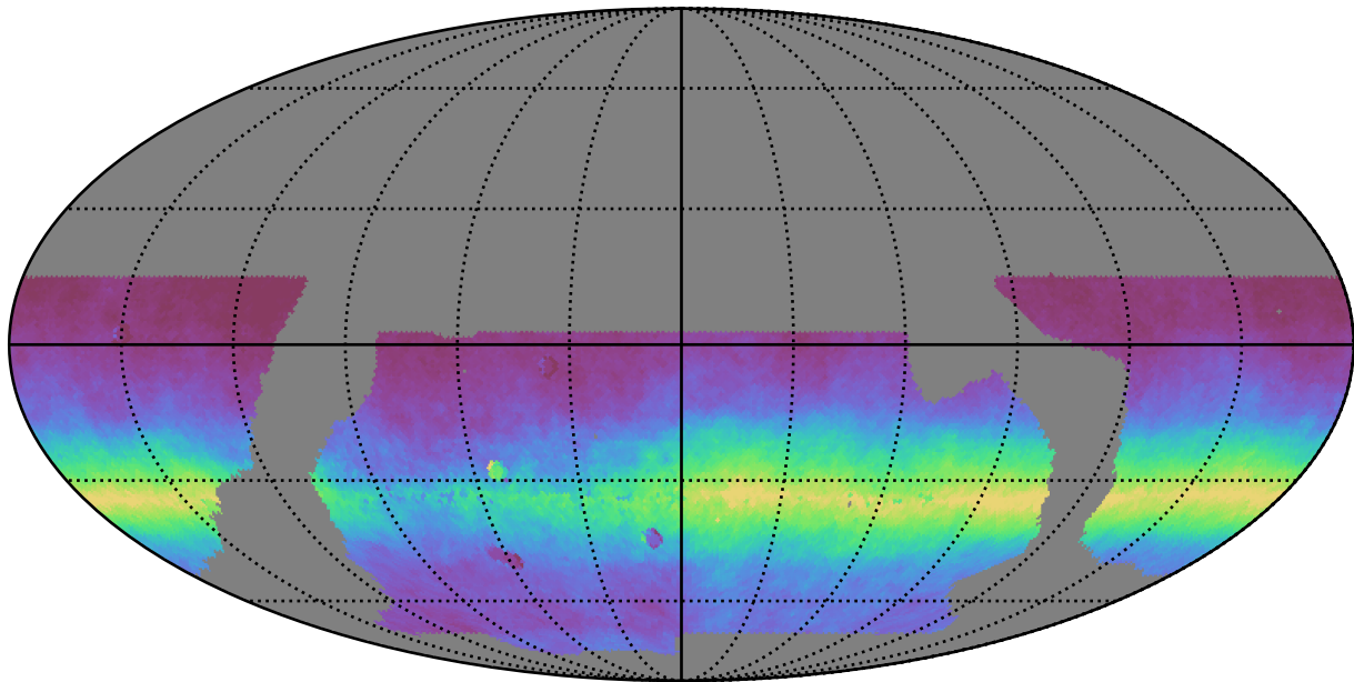
baseline_v2.0_10yrs WFD all bands: AngleRms rotSkyPos
