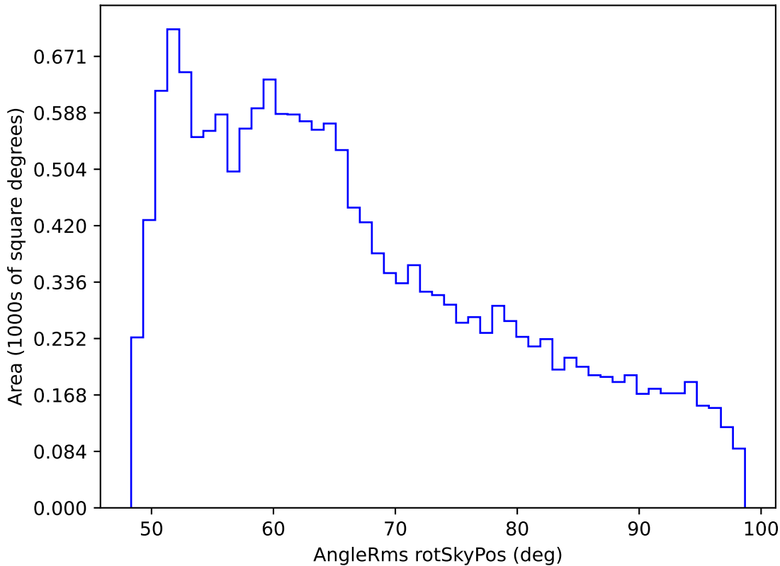
baseline_v2.0_10yrs WFD all bands: AngleRms rotSkyPos
