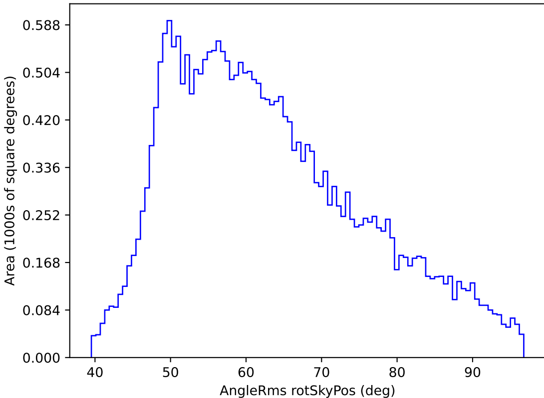
baseline_v2.0_10yrs All sky z band: AngleRms rotSkyPos
