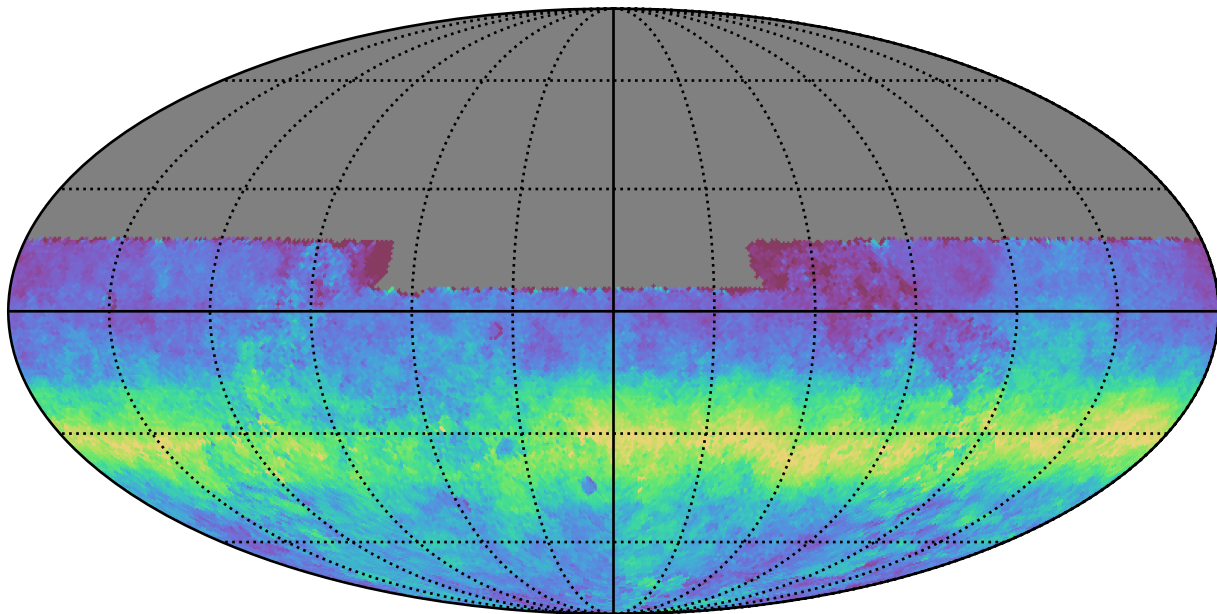
baseline_v2.0_10yrs All sky u band: AngleRms rotSkyPos
